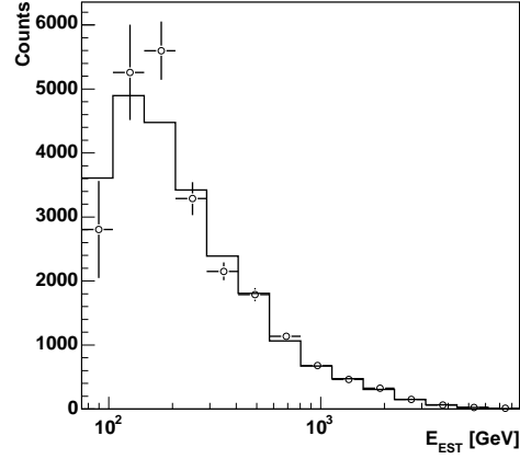
(b) Distribution Y to be unfolded (open circles), and the unfolded distribution S folded with M (histogram)
