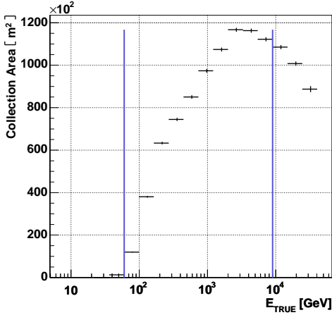
(c) Effective collection area A_{eff}
