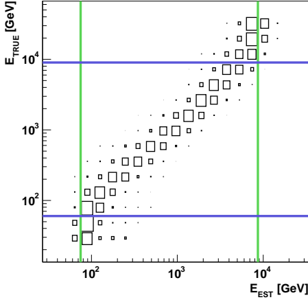
(a) Original migration matrix M
