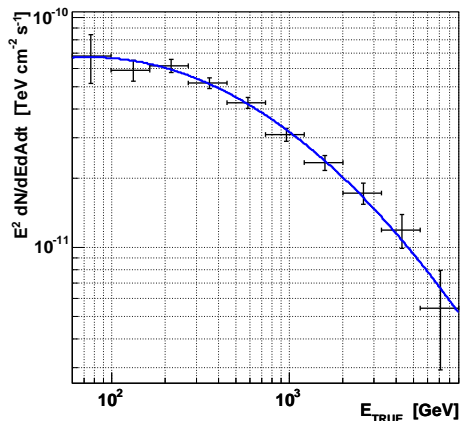
(a) Unfolded distribution S before (grey symbols) and after the correction for the cut in E_{est} (black symbols). (b) Result for the differential \gamma -ray flux \Phi(E_{true}) multiplied with E^2 .
