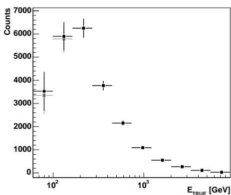
(a) Unfolded distribution S before (grey symbols) and after the correction for the cut in E_{est} (black symbols). (b) Result for the differential \gamma -ray flux \Phi(E_{true}) multiplied with E^2 .
