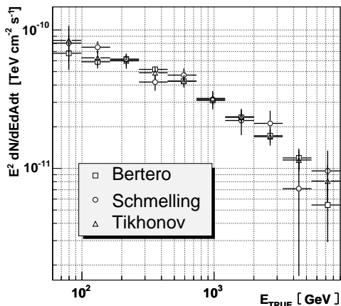
(c) Comparison of the results for E^2 \cdot \Phi(E_{true}) from different unfolding methods.
