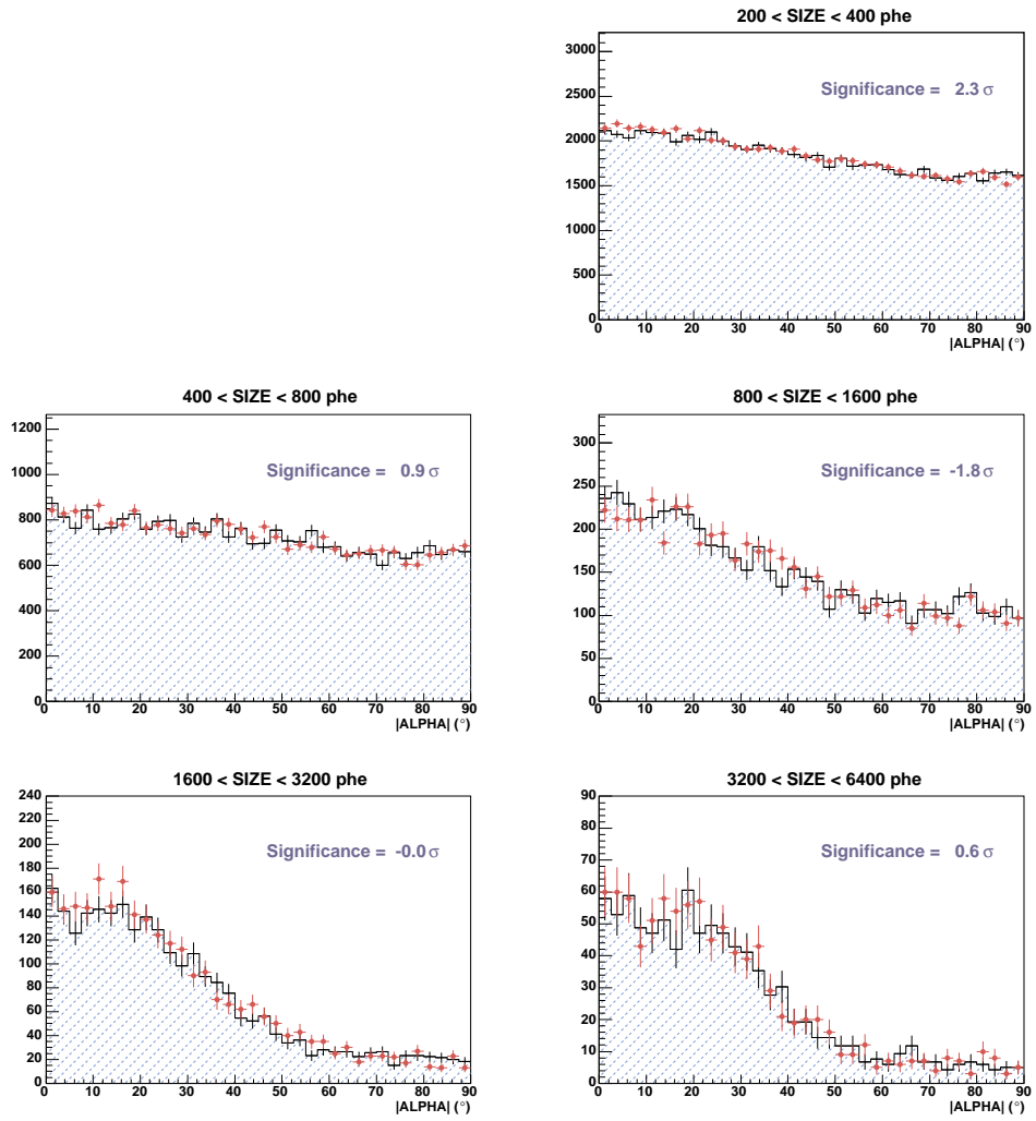
Fig. 1.— ALPHA plots for the Arp 220 data, separated in bins of SIZE.
