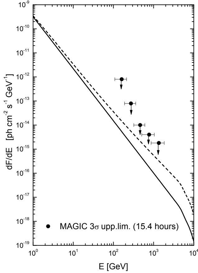
Fig. 2.— MAGIC upper limits to the differential \gamma -ray flux of Arp 220. The curves represent the theoretical predictions, a solid line shows the result using the \delta -function (Aharonian & Atoyan 2000) or Kamae et al. (2005) approximations for the proton-proton cross section, whereas a dashed line shows the result using the parameterization proposed by Blattnig et al. (2000), extrapolated to high energies. Theoretical curves are from (Torres 2004, and Torres & Domingo-Santamaría 2005).
