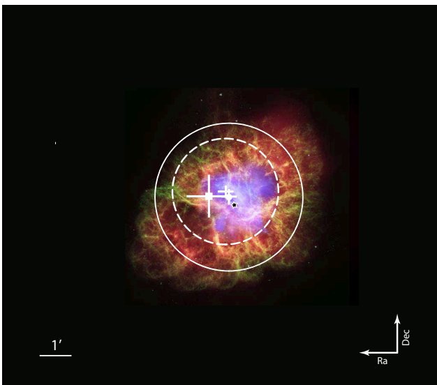
FIG. 16.— Emission of the Crab Nebula in different energy bands. The position of the Crab pulsar is marked with a black star. The Chandra X-ray image is shown in light blue, the Hubble Space Telescope optical images are in green and dark blue, and the Spitzer Space Telescope's infrared image is in red (picture from Chandra 2006). Overlaid are the center of gravity of the \gamma -ray emission at different energies (simple cross > 500 GeV; dot \sim 250 GeV; square \sim 160 GeV). The error bars indicate the statistical uncertainty in the position of the CoG. The upper limits (95% confidence level) on the 39% containment radius of the \gamma -ray emission region that were derived from the \theta^2 -distributions are indicated with circles (dashed > 500 GeV; solid \sim 250 GeV).
