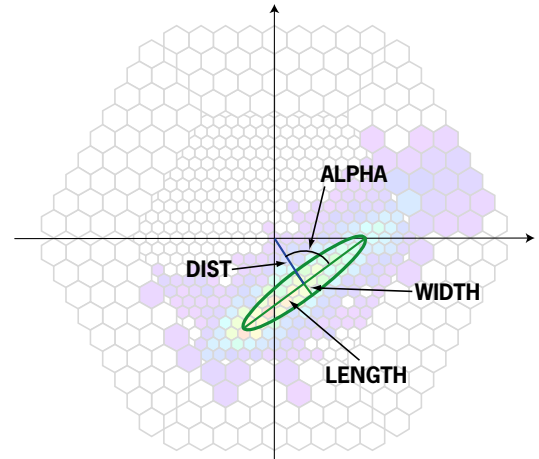
FIG. 1.— Parameterization of a shower image with Hillas-parameters.
