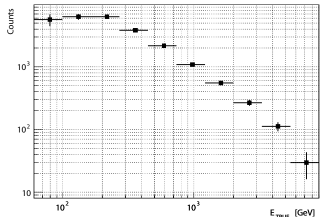
FIG. 8.— Unfolded distribution of excess events from the Crab Nebula. The integral rate of excess events is 0.4 Hz.
