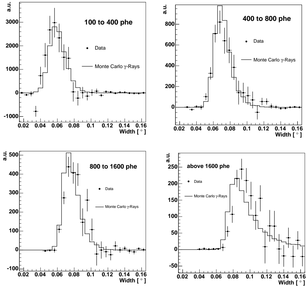
FIG. 3.— Distribution of the image parameter WIDTH for \gamma -ray events extracted from data and for Monte Carlo simulated \gamma -rays in four consecutive bins of SIZE covering the full analyzed energy range. Data and Monte Carlo show good agreement in all four bins.
