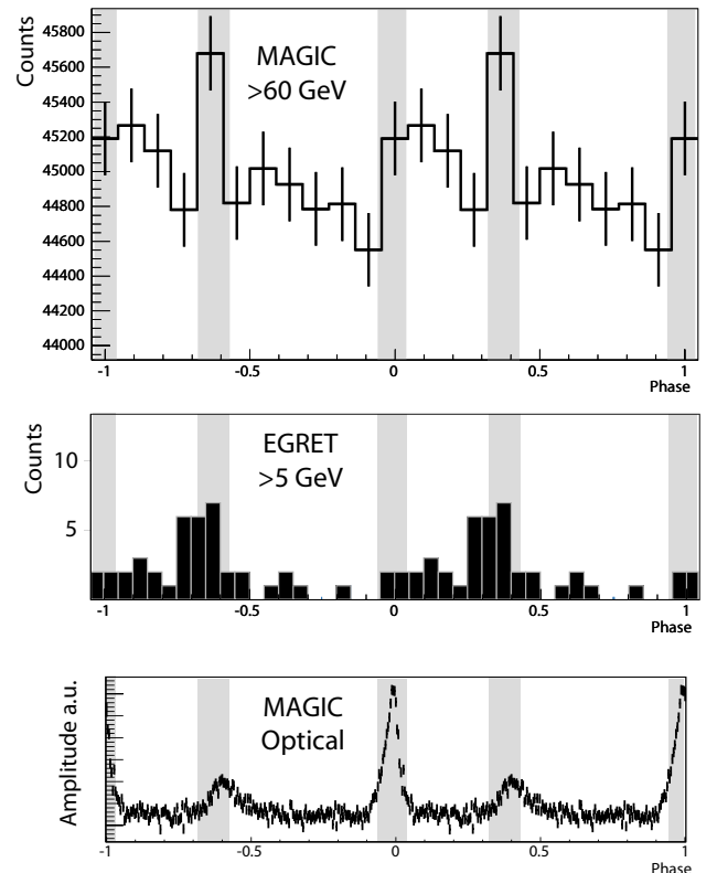
FIG. 20.— Pulse phase profiles of the Crab pulsar. Lower figure: optical observations by MAGIC ( \sim 1 s effective observation time); middle figure: observations by EGRET above 5 GeV; upper figure: pulse phase profile obtained by MAGIC, analysis threshold 60 GeV. The shaded regions indicate the EGRET measured positions of the peaks for \gamma -ray energies above 100 MeV.
