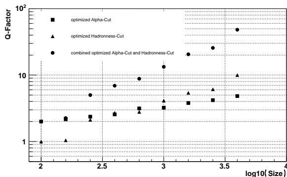
FIG. 6.— Size dependence of the Q-factor for optimized |\text{ALPHA}| -cut, HADRONNESS-cut and the Q-factor for the combination of |\text{ALPHA}| -cut and HADRONNESS-cut.
