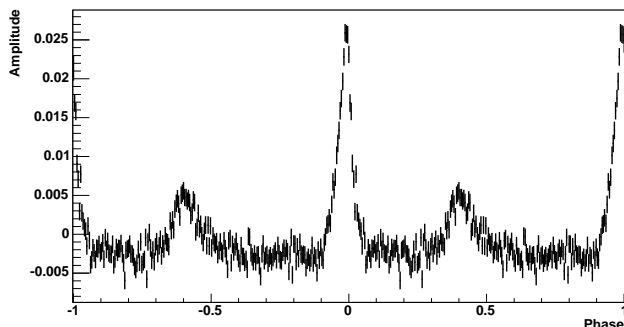
FIG. 18.— Optical light curve of the Crab pulsar measured with MAGIC. The figure includes data from seven different observations between December 2005 and February 2006. The total observation time was 12.5 hours.
