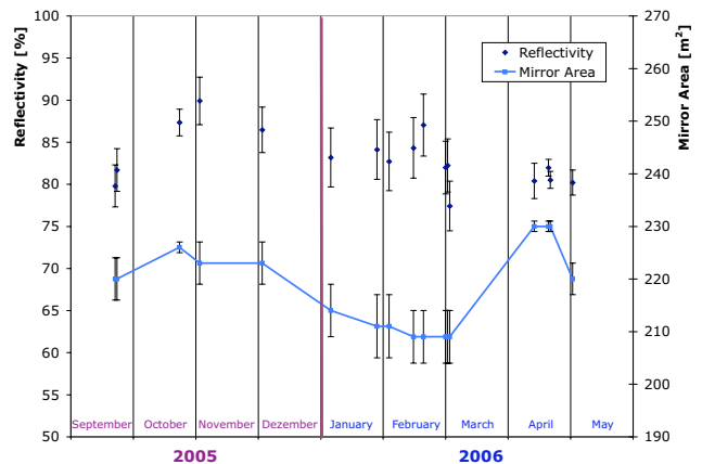
FIG. 7.— Measurement of the reflectivity of the main mirror (Garczarczyk 2006). The measurements cover the Crab observation period from Oct. to Dec. 2005
