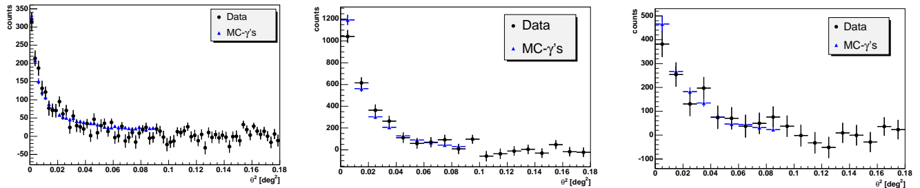
FIG. 17.— Background subtracted \theta^2 -distributions for different energies. From left to right > 500 GeV, \sim 250 GeV, \sim 160 GeV
