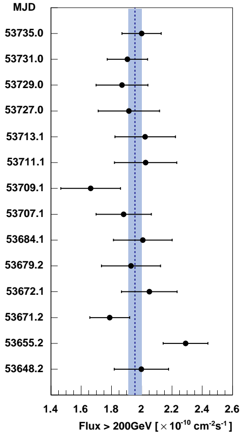
FIG. 14.— Nightly average flux from the Crab Nebula above 200GeV of each observed night. The dashed blue line gives the average flux of all nights and the blue shaded region the corresponding statistical error.
