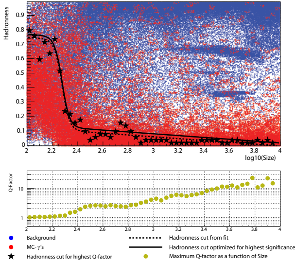
FIG. 4.— Upper figure: Distribution of the parameter HADRONNESS vs. SIZE. The background events are marked blue and the MC \gamma -ray events red. Note that below a SIZE of 300 phe most of the background events are hidden behind the simulated \gamma -ray events. For bins in SIZE the HADRONNESS cuts that yield the highest quality factors (black stars) are found. The solid black line is a fit to the HADRONNESS values. Lower figure: Quality factor for the HADRONNESS-cut in the upper figure.
