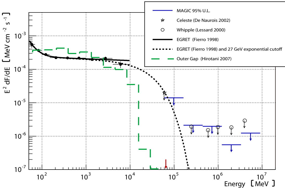
FIG. 19.— Upper limits on the pulsed gamma ray flux from the Crab pulsar; upper limits in differential bins of energy are given by the blue points. The upper limit on the cutoff energy of the pulsed emission is indicated by the dashed line. The analysis threshold to derive the upper limit on the cutoff energy is indicated by the red arrow.
