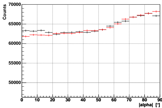
FIG. 5.— Distribution of the parameter |\text{ALPHA}| for the bin of reconstructed energy 80...100 GeV in the left panel and for events with energies > 200 GeV in the right panel.
