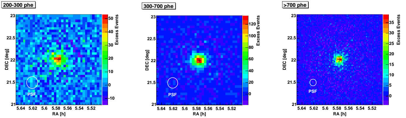
FIG. 15.— Sky-maps of excess events from the Crab Nebula for different \gamma -ray energies ( \sim 160 GeV, \sim 250 GeV and > 500 GeV). The position of the pulsar is marked by the black cross and the angular resolution is indicated by the circle.
