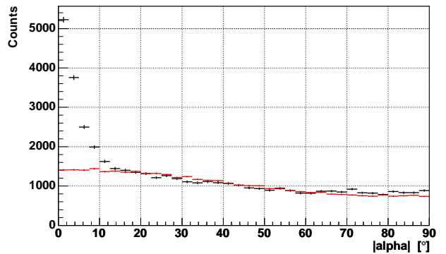
FIG. 5.— Distribution of the parameter |\text{ALPHA}| for the bin of reconstructed energy 80...100 GeV in the left panel and for events with energies > 200 GeV in the right panel.
