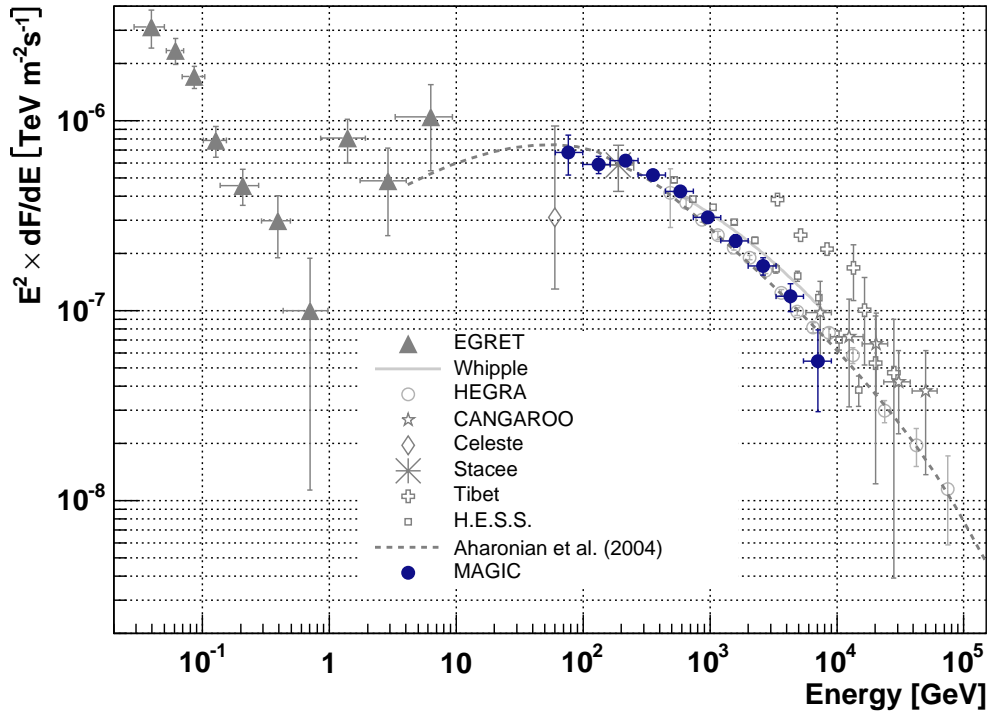
FIG. 11.— Spectral energy distribution of the \gamma -ray emission of Crab Nebula. The measurements shown below 10 GeV are by EGRET. In VHE \gamma -rays, measurements are from ground-based experiments. Above 400 GeV our measurement is in agreement with measurements by other IACTs. The dashed line is a model prediction by Aharonian et al. (2004).
