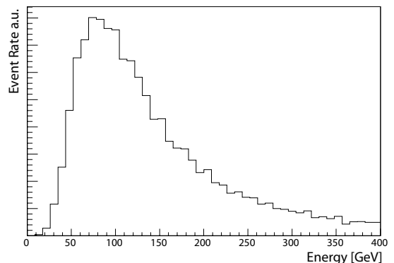
FIG. 2.— Energy distribution of MC- \gamma -ray events with SIZE > 100 phe.
