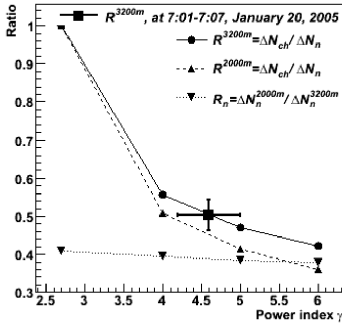
Figure 6 Estimation of the energy Spectra index by comparing different secondary fluxes measured at same the location
