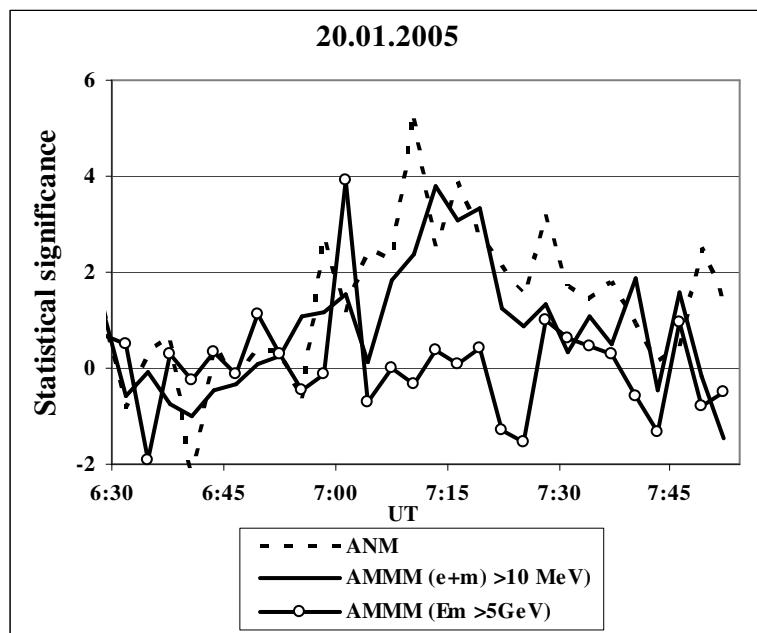
Figure 4 Detection of the GLE from 20 January 2005 by ASEC monitors
