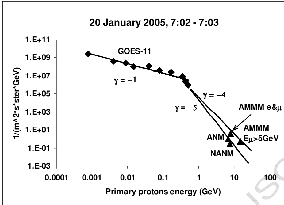
Figure 5 Differential energy spectra of the SCR protons 20 January 2005
