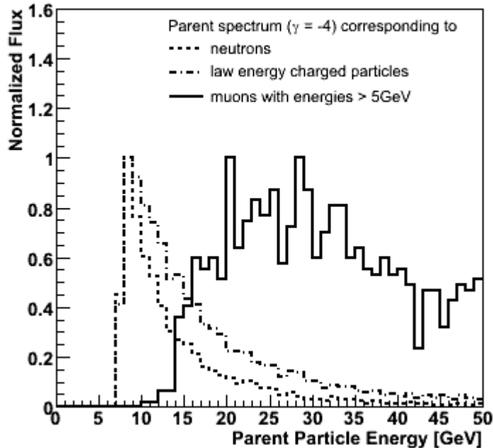
Figure 3 Simulation of the “Parent” energy spectra of secondary particles initiated by the SCR (spectral slope equals -4), “selected” by the ASEC monitors at 3200 m.
