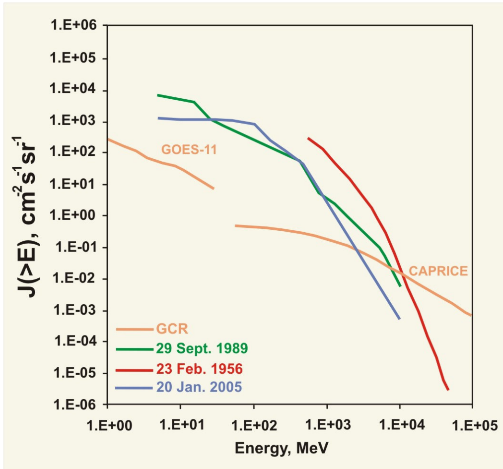
Figure 1 Galactic and Solar Cosmic Rays
