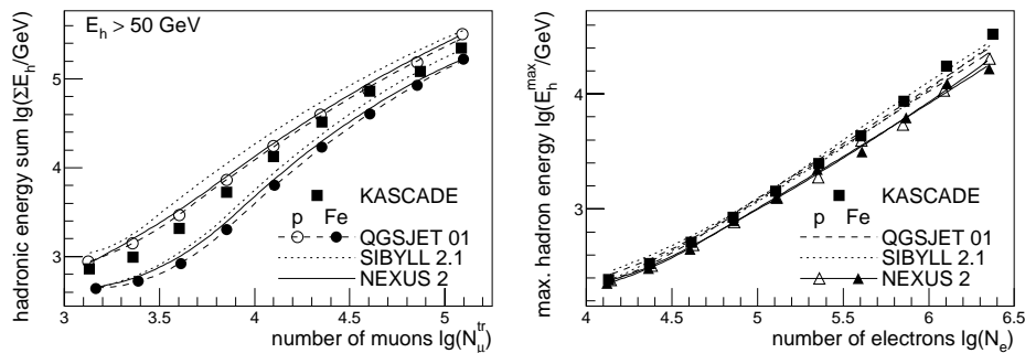
Fig. 1. Left-hand side: Correlation between the hadronic energy sum \Sigma E_h and the number of muons N_\mu^{\text{tr}} . Right-hand side: Correlation of the most energetic hadron E_h^{\max} and the number of electrons N_e . To improve the visibility, for some of the models only parameterizations are shown.
