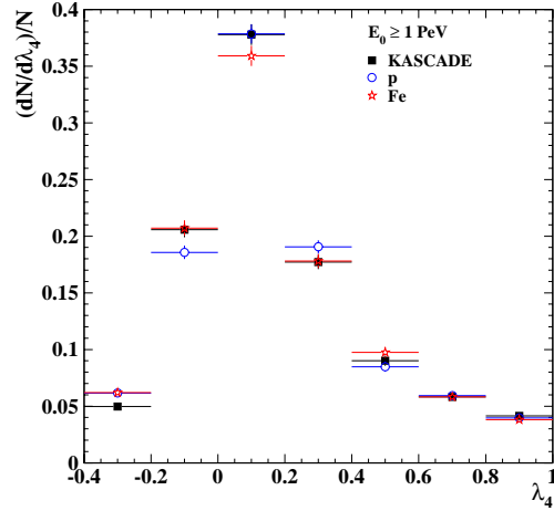
Fig. 3. Distributions of the alignment parameter \lambda_4 . KASCADE measurements are compared with QGSJET 01 simulations.
