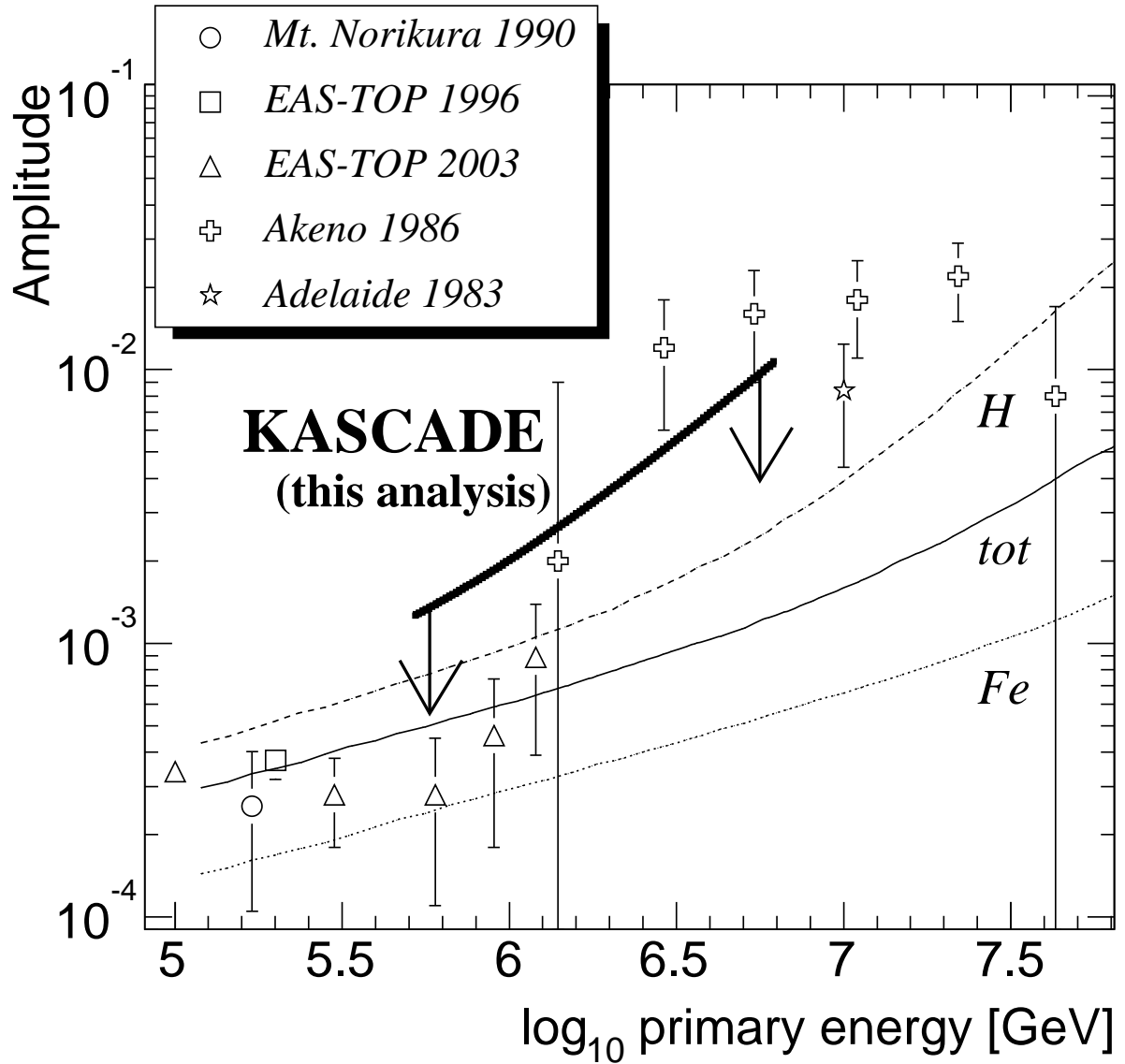
Fig. 6.— KASCADE upper limits (95%) of Rayleigh amplitudes A vs. primary energy (bold line) compared to reported results from literature (Nagashima et al. 1990; Aglietta et al. 1996, 2003; Kifune et al. 1986; Gerhardy & Clay 1983). Model predictions from Candia, Mollerach, & Roulet (2003) for the total anisotropy and for anisotropies of the proton and iron component are shown as well (thin lines).
