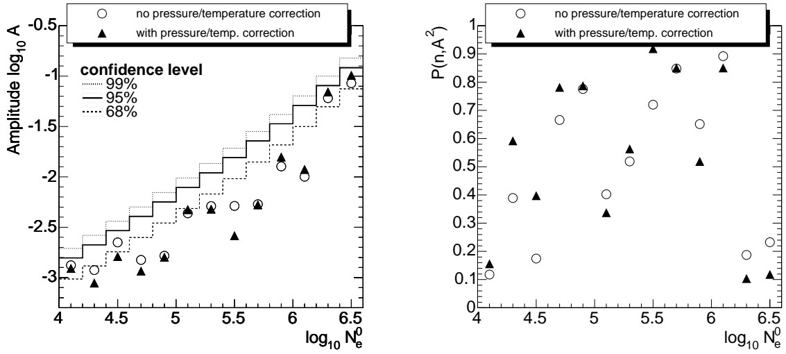
Fig. 4.— Result from the Rayleigh analysis for showers without and with correction for atmospheric ground pressure and temperature. Left-hand side: Rayleigh amplitude A vs. electron number \log_{10} N_e^0 . Right-hand side: Probability P(n, A^2) that the amplitudes plotted in the left figure are fluctuations from underlying uniform distributions.
