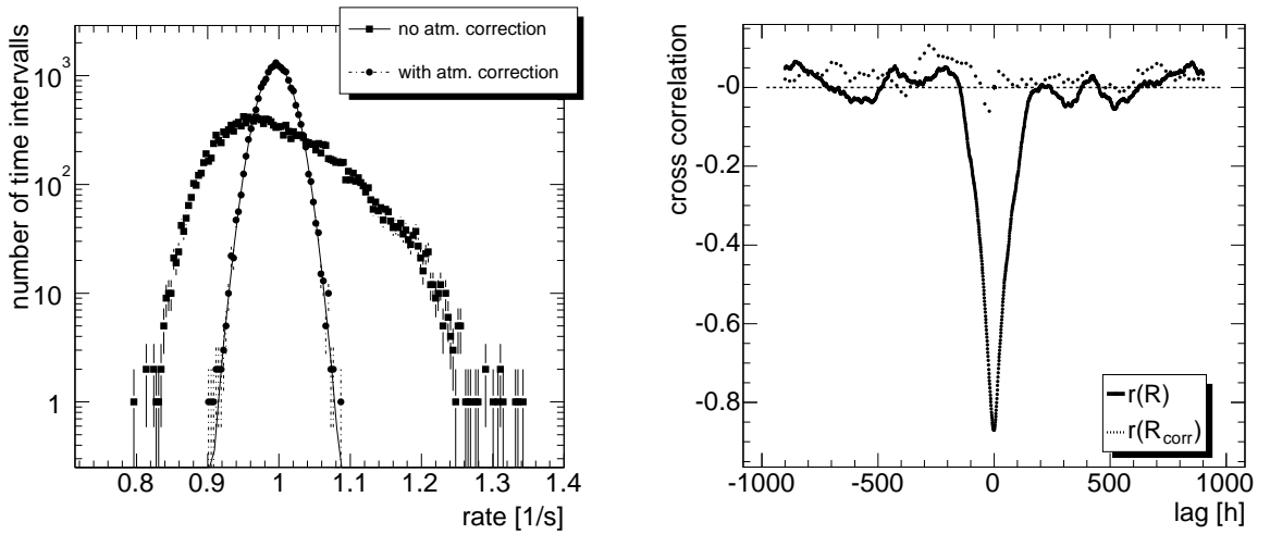
Fig. 2.— Left: Distribution of rates with and without correction for atmospheric ground pressure and temperature. A fit by a Gaussian function is shown by the line. Right: Cross correlation between hourly shower rate and atmospheric ground pressure with ( r(R_{corr}) ) and without atmospheric correction ( r(R) ).
