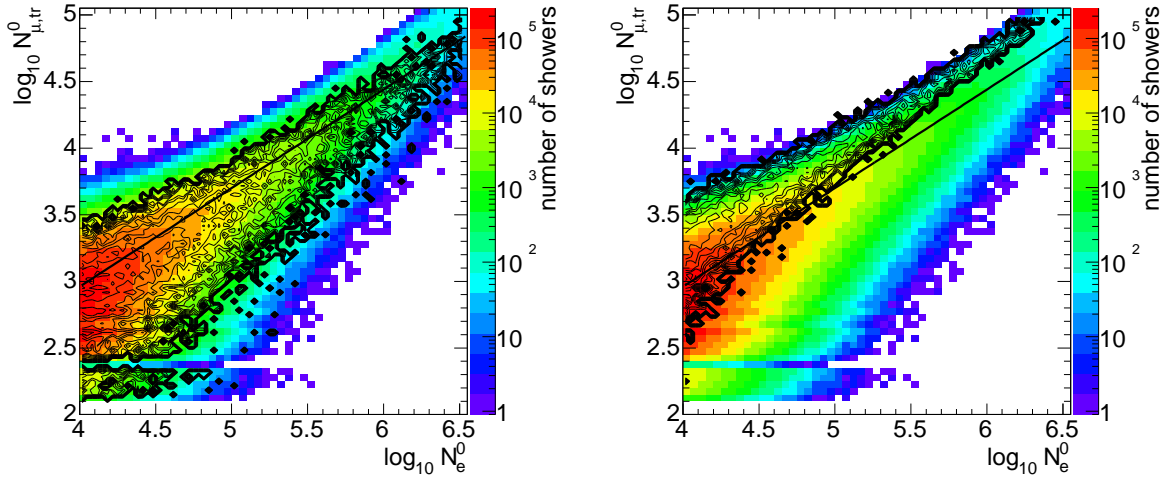
Fig. 1.— Number of muons versus number of electrons ( \log_{10} N_{\mu, tr}^0 vs. \log_{10} N_e^0 ) of showers measured with KASCADE (shaded area). Simulated air showers induced by primary protons (left-hand side) or iron nuclei (right-hand side) are superimposed (contour lines). The straight lines in both figures indicate the separation between light and heavy primaries according to equation 4.
