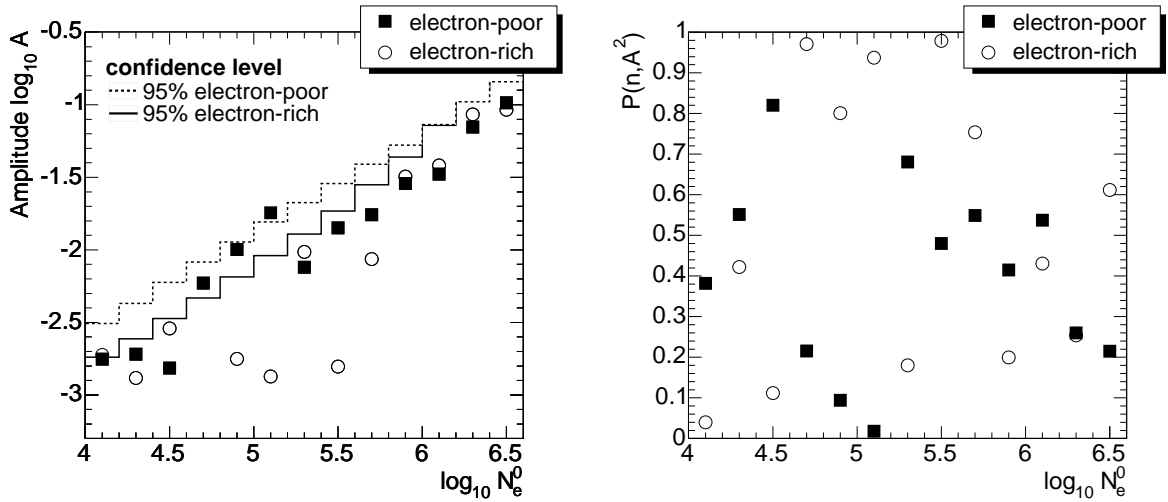
Fig. 5.— Result from the Rayleigh analysis for data sets of predominately light and heavy primaries. Left-hand side: Rayleigh amplitude A vs. electron number \log_{10} N_e^0 . Right-hand side: Probability P(n, A^2) that the amplitudes in the left figure are fluctuations from underlying uniform distributions.
