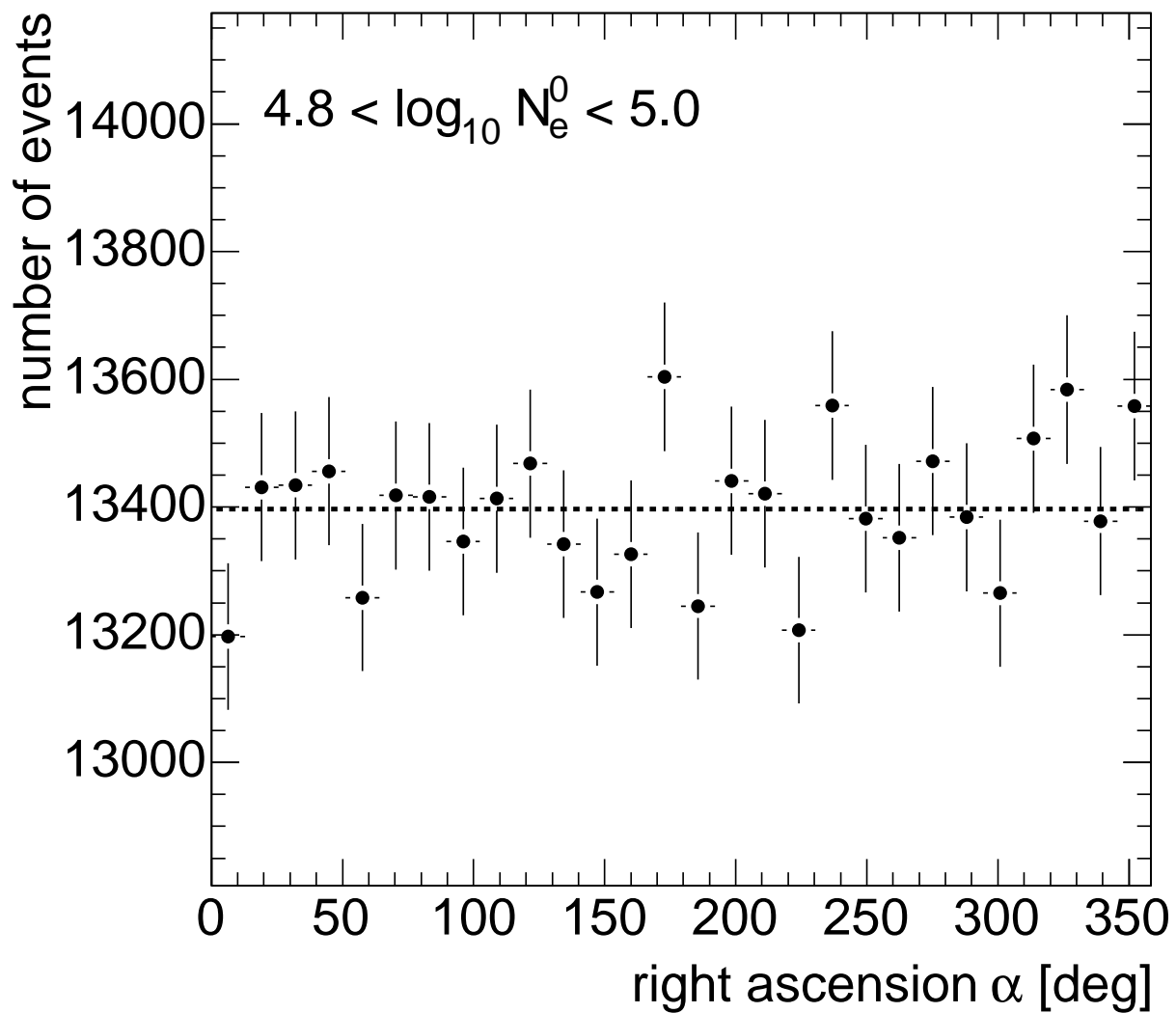
Fig. 3.— Example of a right ascension distribution after correction for atmospheric ground pressure and temperature in the stated electron number interval. The dashed line reflects the mean number of events.
