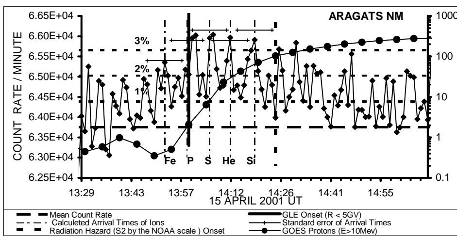
Figure 3. The 15 April 2001 GLE. Estimated arrival times of relativistic ions superimposed on the ANM 1 minute time series. Horizontal dashed lines indicate 1, 2 and 3% enhancements relative to mean count rate.
