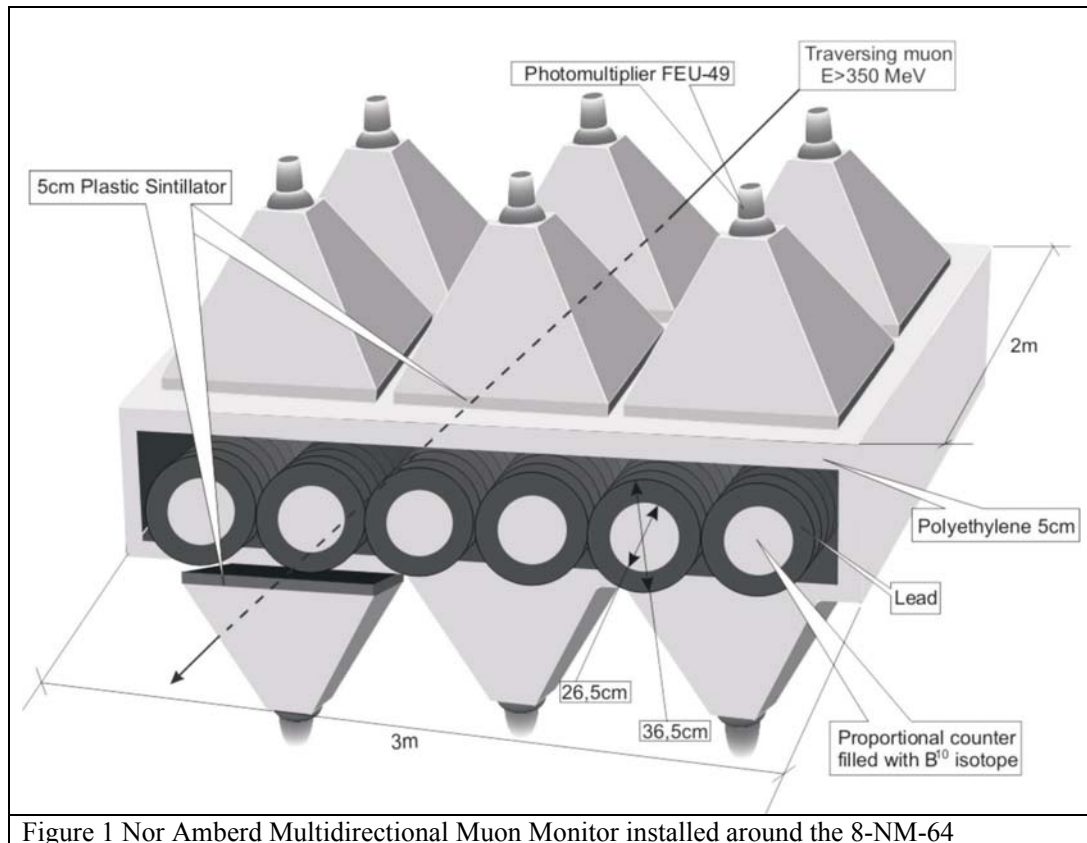
Figure 1 Nor Amberd Multidirectional Muon Monitor installed around the 8-NM-64
