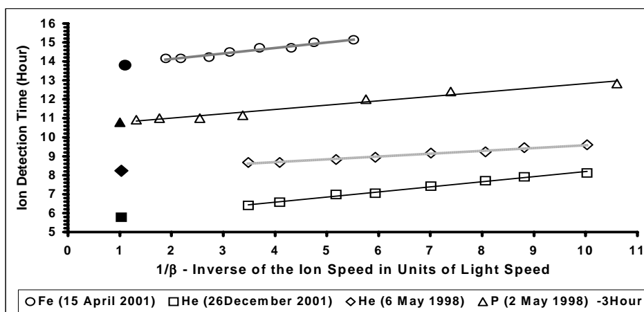
Figure 2. Linear correlation of ion arrival times to 1 AU versus their inverse speed. The filled symbols correspond to the expected arrival times of relativistic ions. The proton event is shifted down by 3 hours for better visualization of the regression lines.
